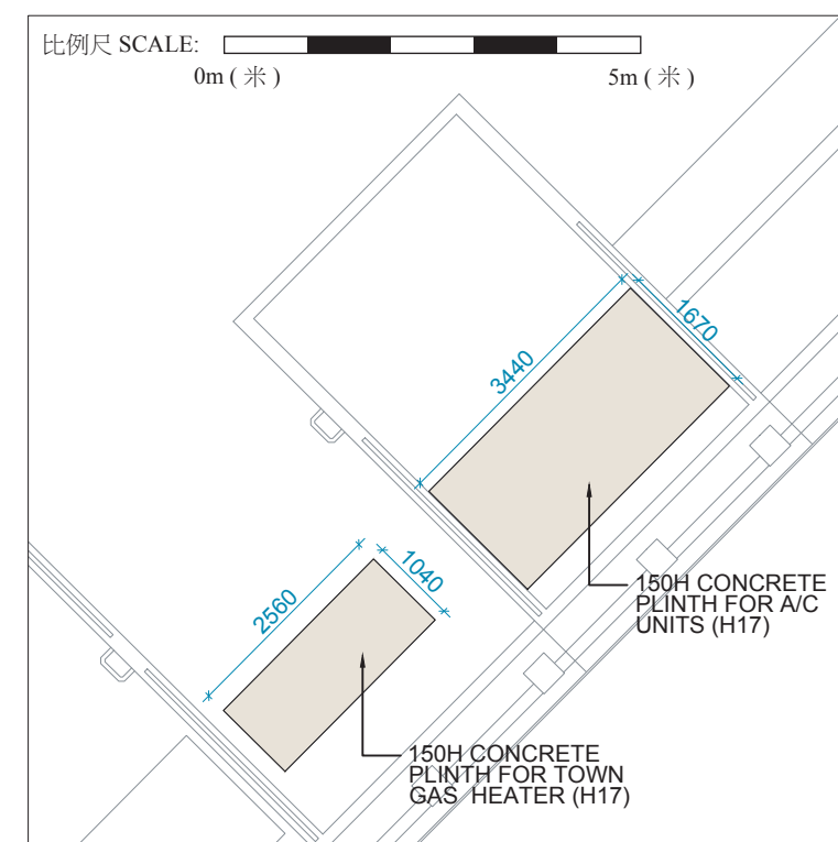
17 號洋房地主層部分平面圖 Part Plan For House 17 Master Ground Floor Plan
